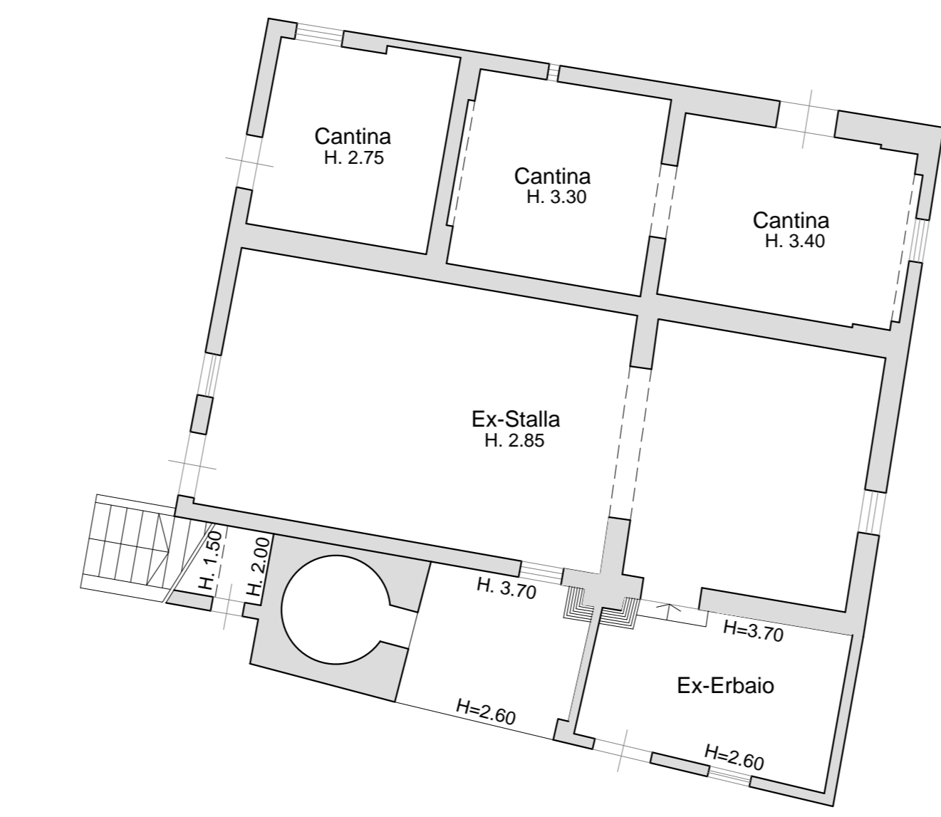
PIANO TERRA
